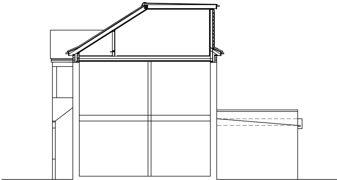
PROPOSED SECTION ELEVATION
