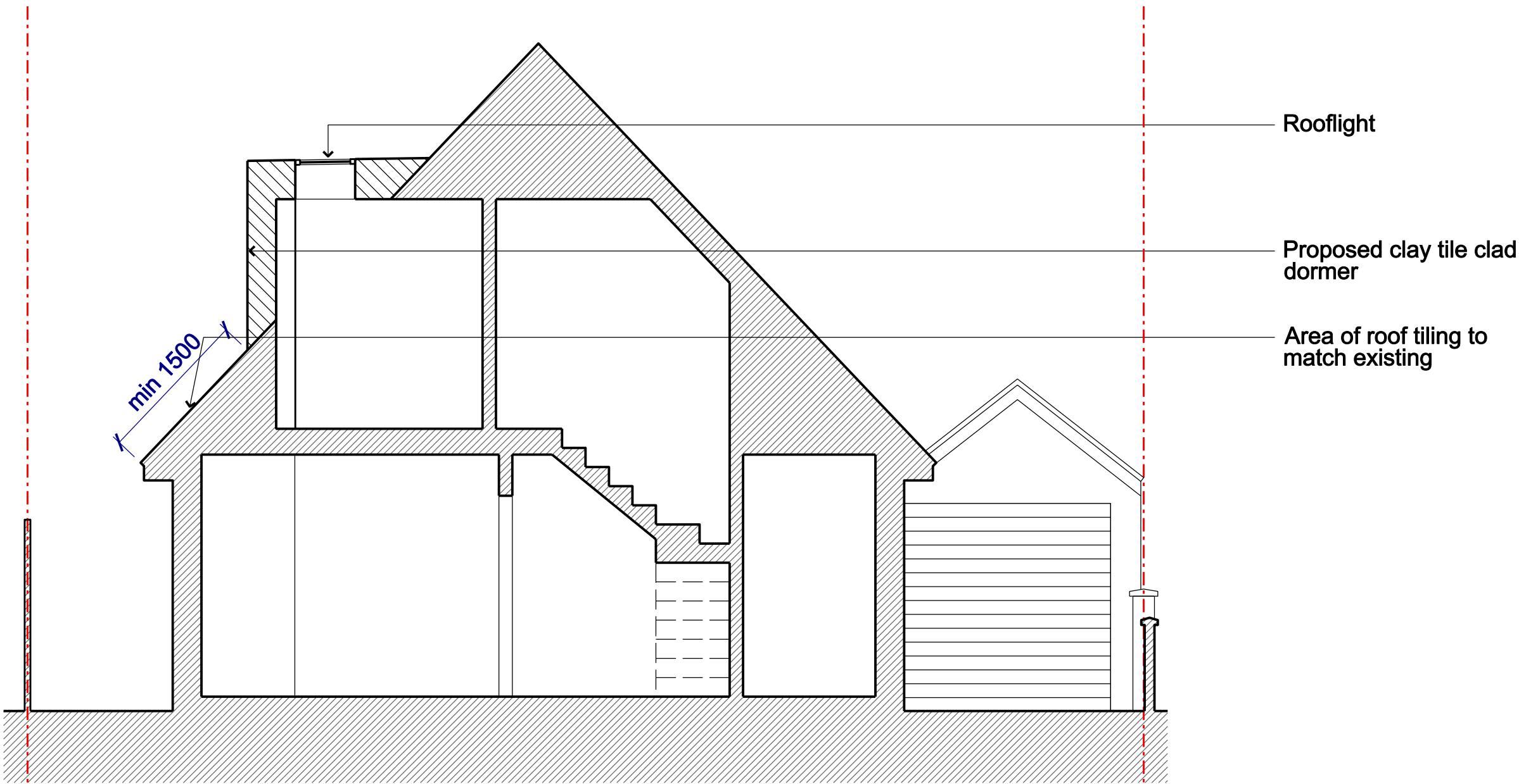
Proposed Section AA 01 500
