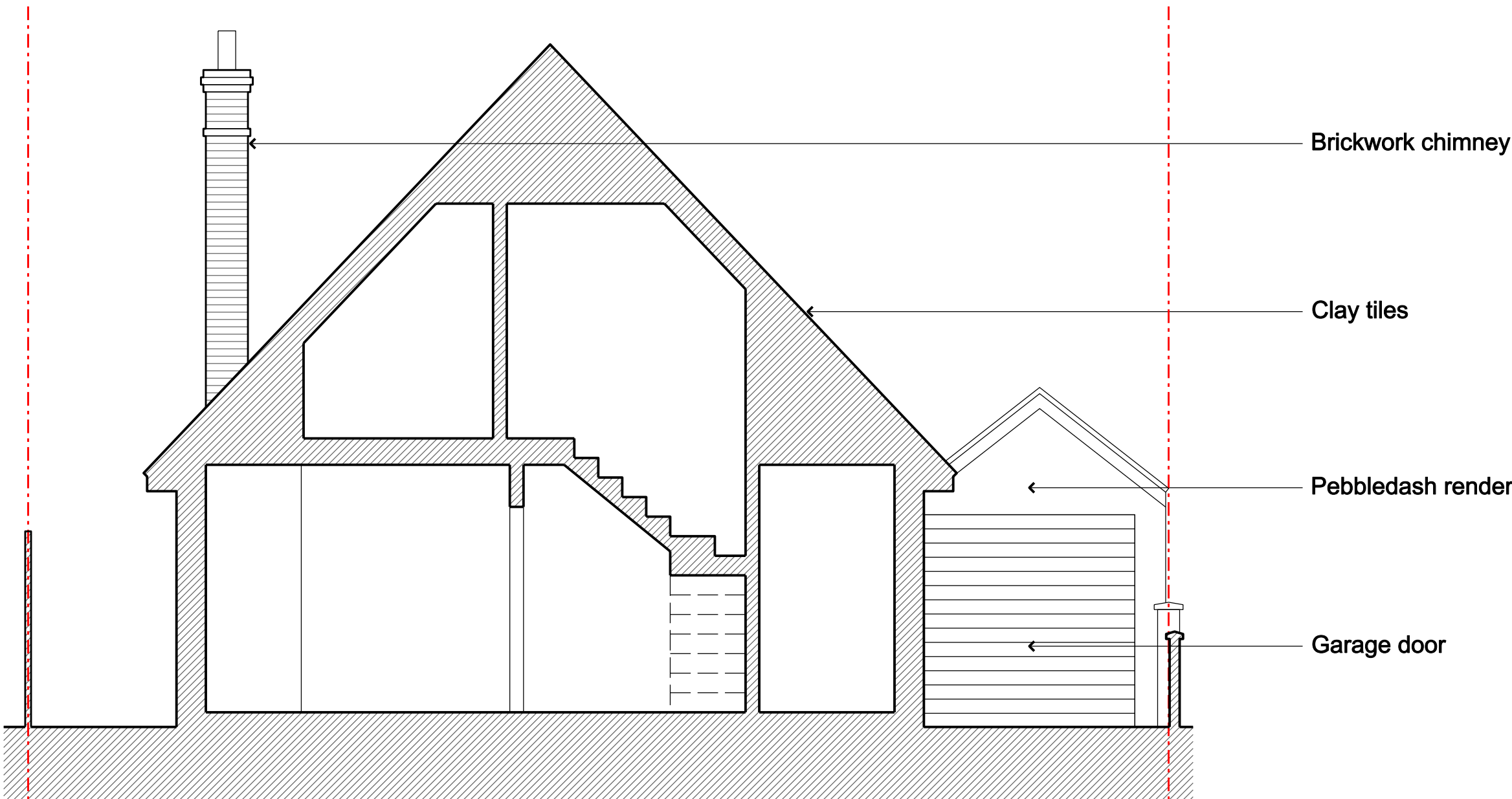
Existing Section AA 01050
