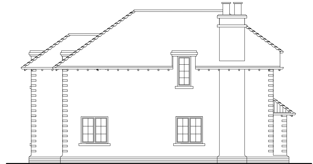
PRE-EXISTING SIDE ELEVATION 1:100
