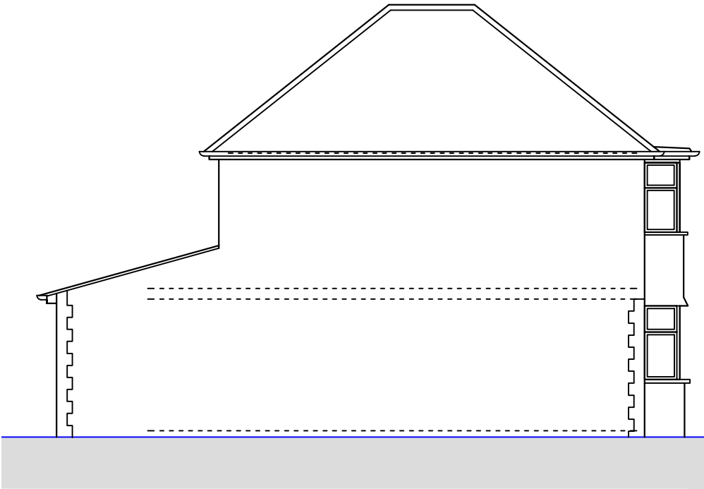
○ Side Elevation 2 1 : 1 0 0
