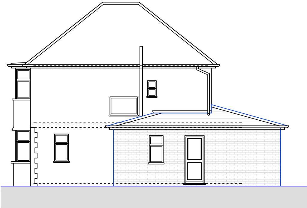
○ Side Elevation 1 1 : 1 0 0
