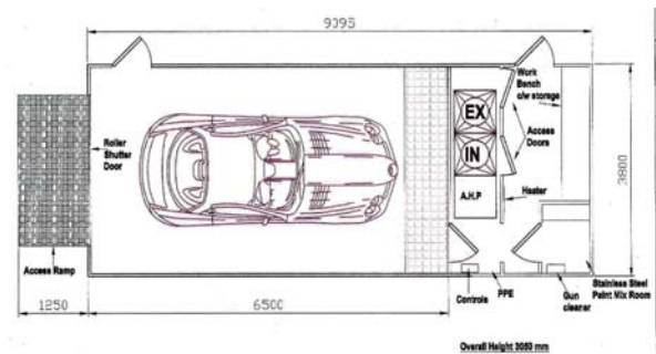
Smartshop general layout
