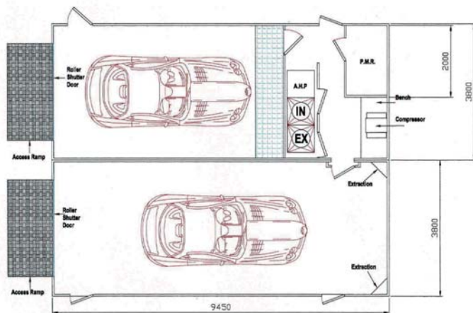
Smartshop and full length prep bay
