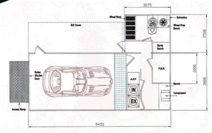
Smartshop plus wheel prep area
