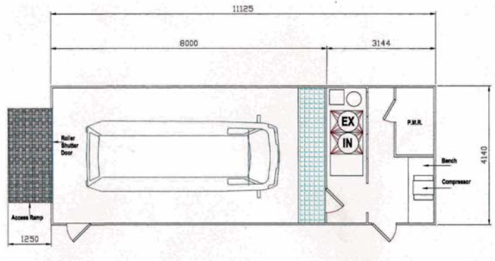
Smartshop for light commercials
