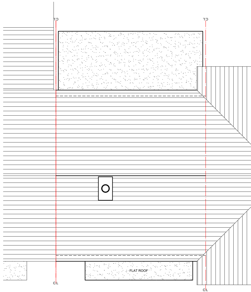
05 - ROOF PLAN
