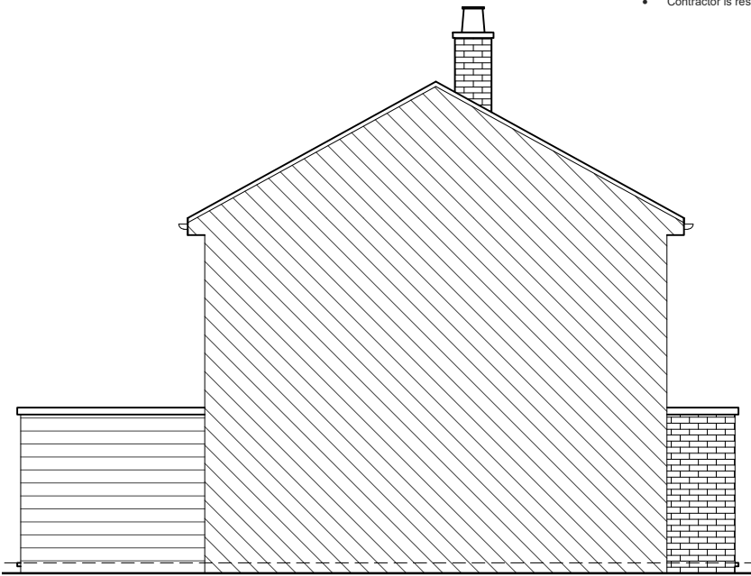
03 - SIDE ELEVATION
