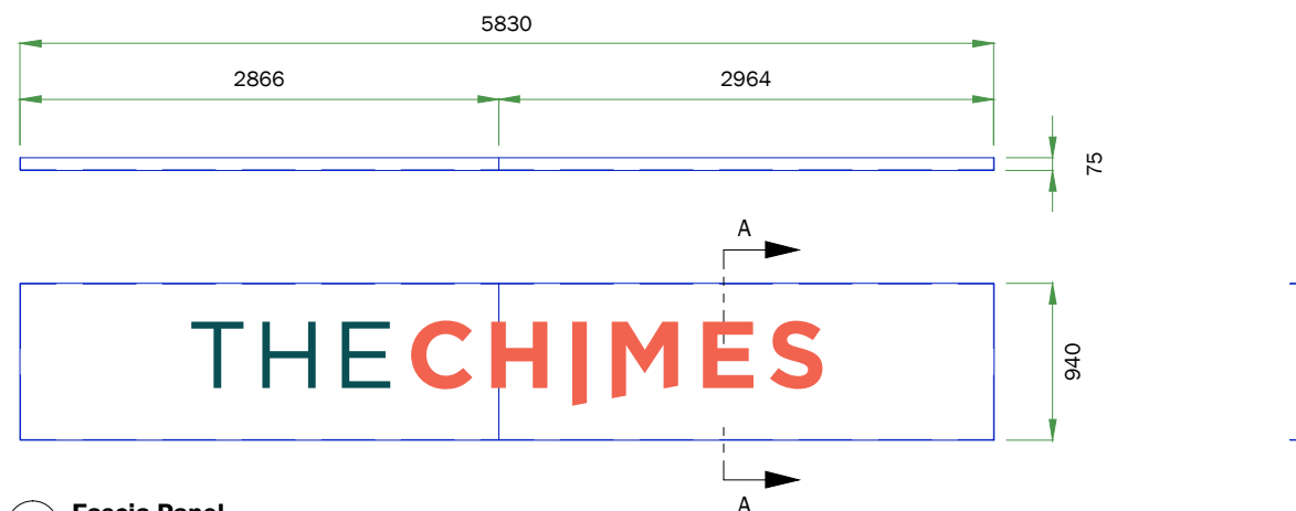
1 Fascia Panel
