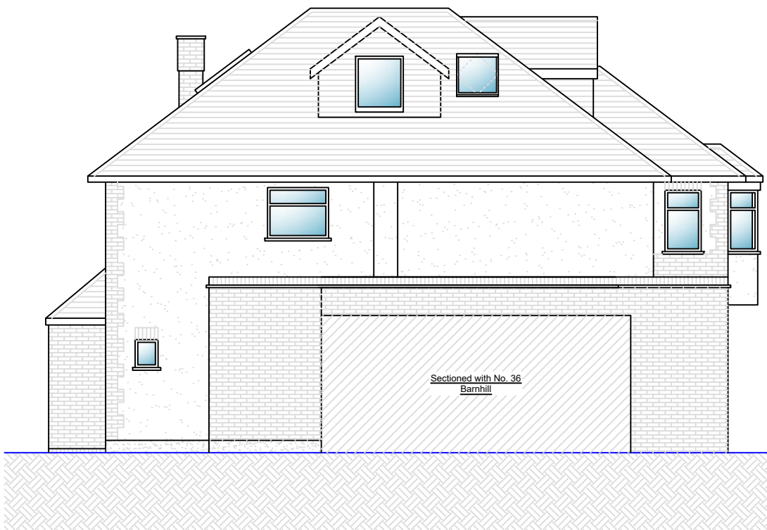
○ Side Elevation 1 1:100
