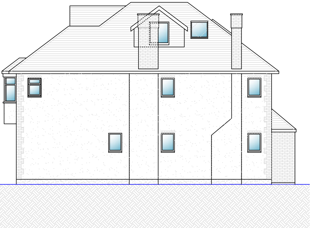
○ Side Elevation 2 1:100
