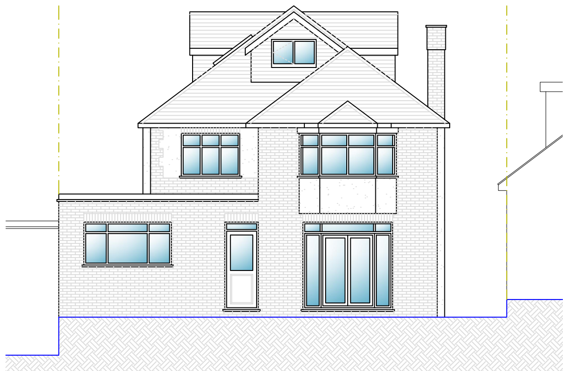
○ Rear Elevation 1 : 1 0 0
