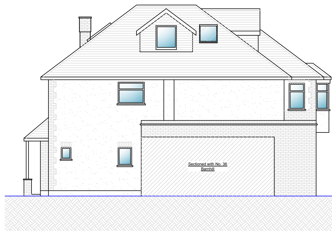
○ Side Elevation 1 1 : 1 0 0
