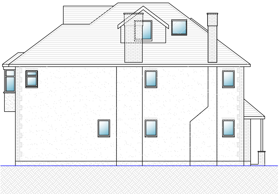
○ Side Elevation 2 1 : 1 0 0
