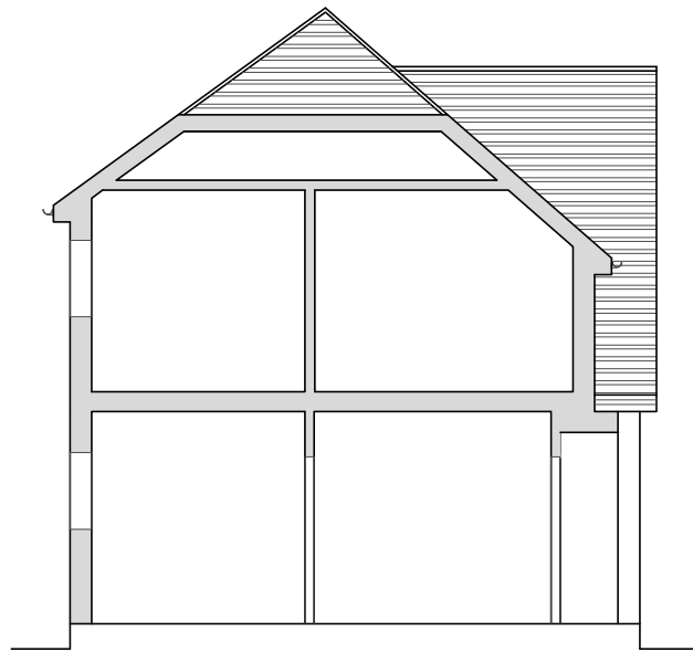
SECTION
