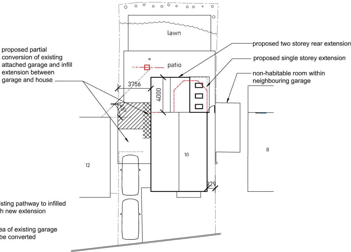
PROPOSED DWELLING SITE LAYOUT PLAN
