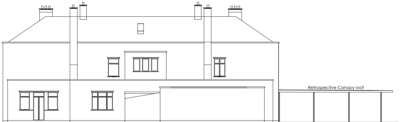
Proposed Rear Elevation - 1:200
