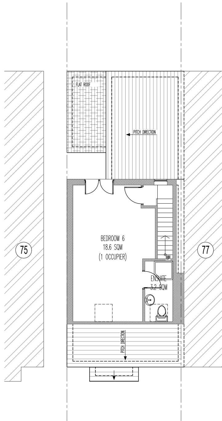
PROPOSED LOFT PLAN SCALE 1/100
