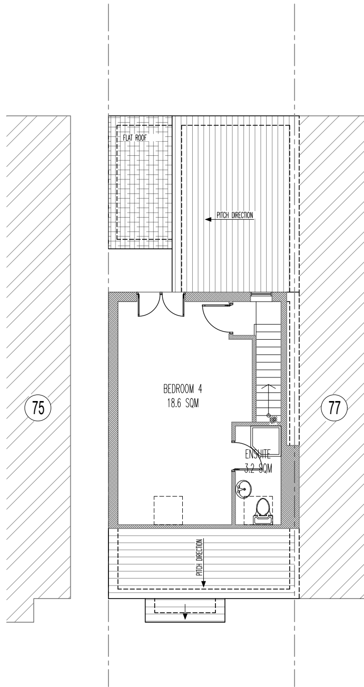
EXISTING LOFT PLAN SCALE 1/100
