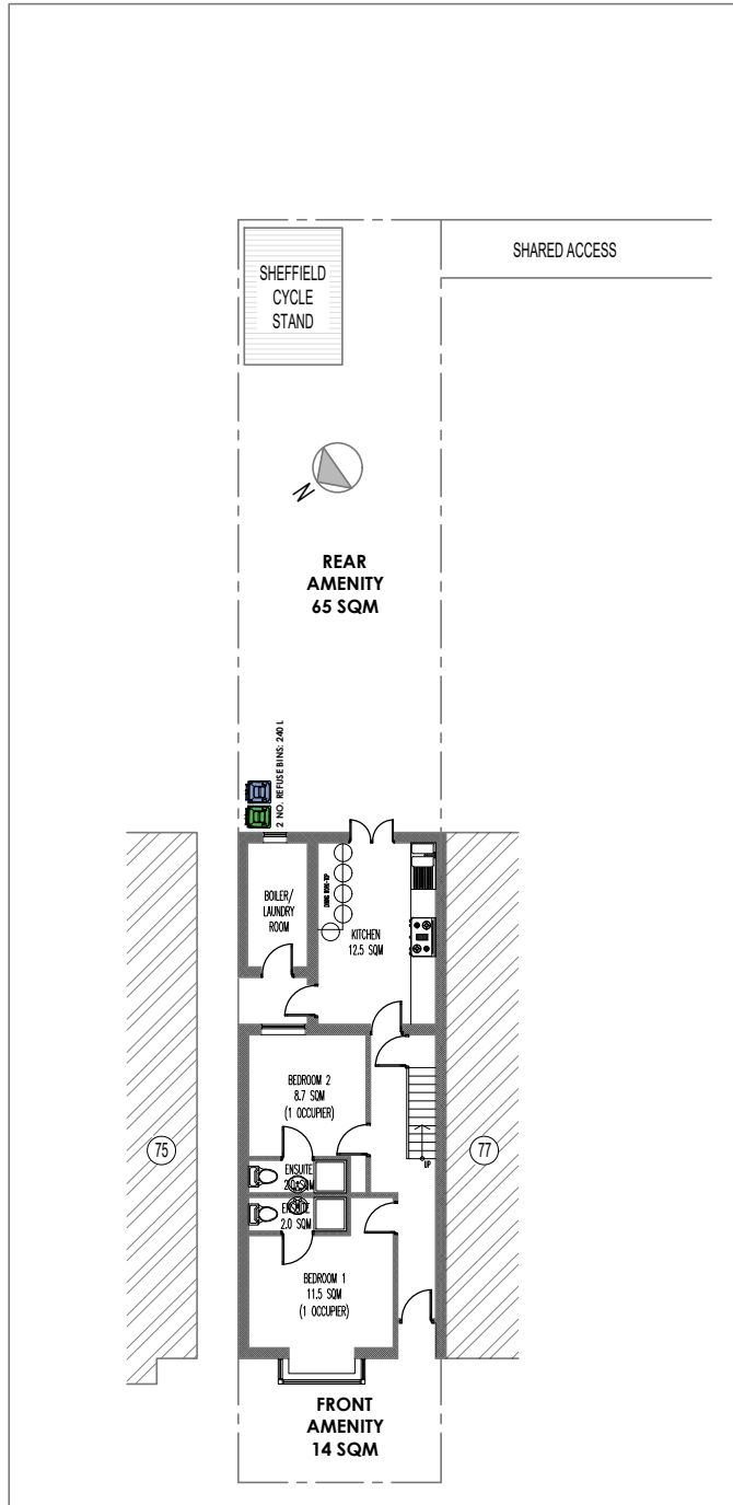
PROPOSED BLOCK PLAN SCALE 1/200
