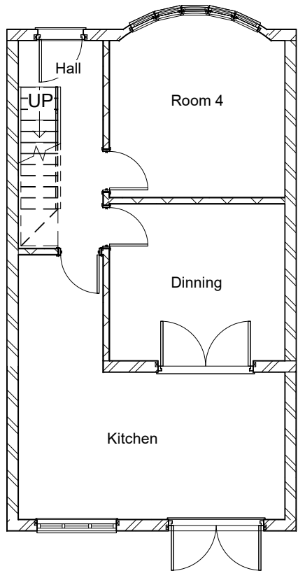
1 Ground Floor 1 : 100
