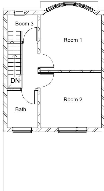
2 First Floor 1 : 100
