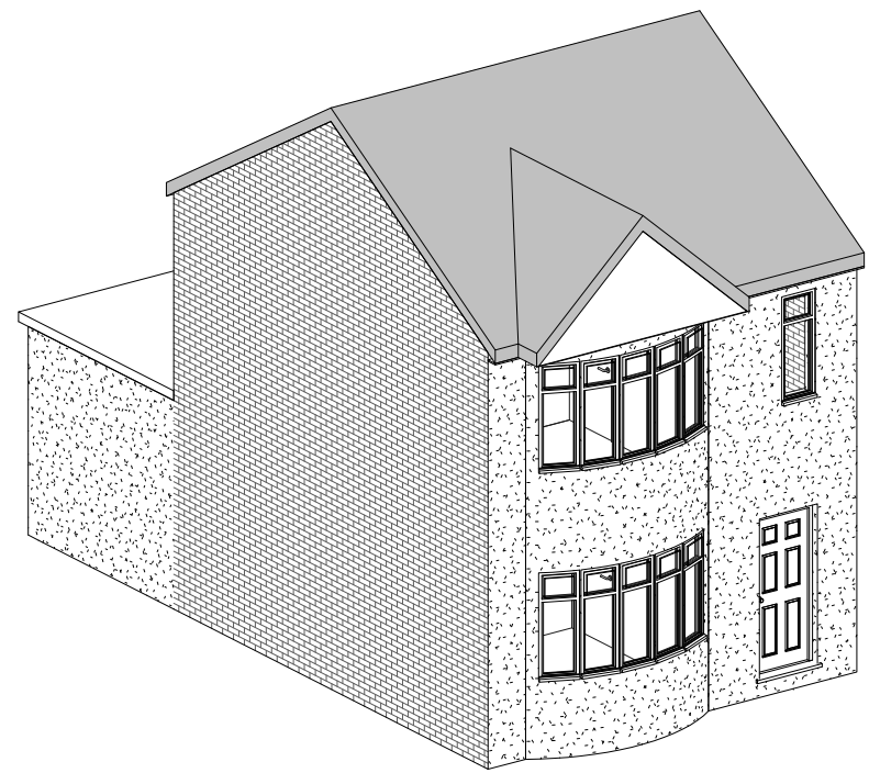
5 Isometric View (Front)
