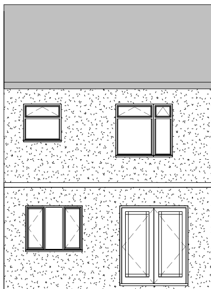
3 South (Rear) Elevation 1 : 100
