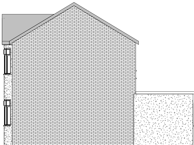
4 West (Flank) Elevation 1 : 100
