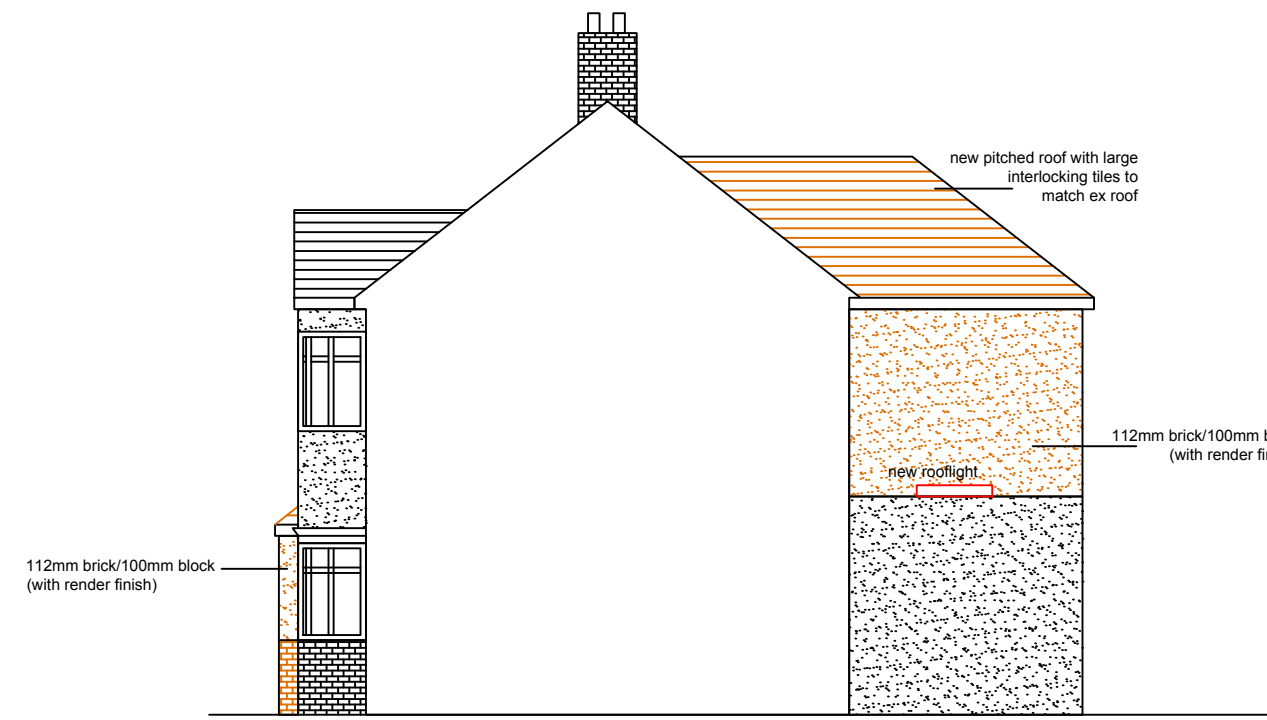
proposed side elevation from no.55 1:100
