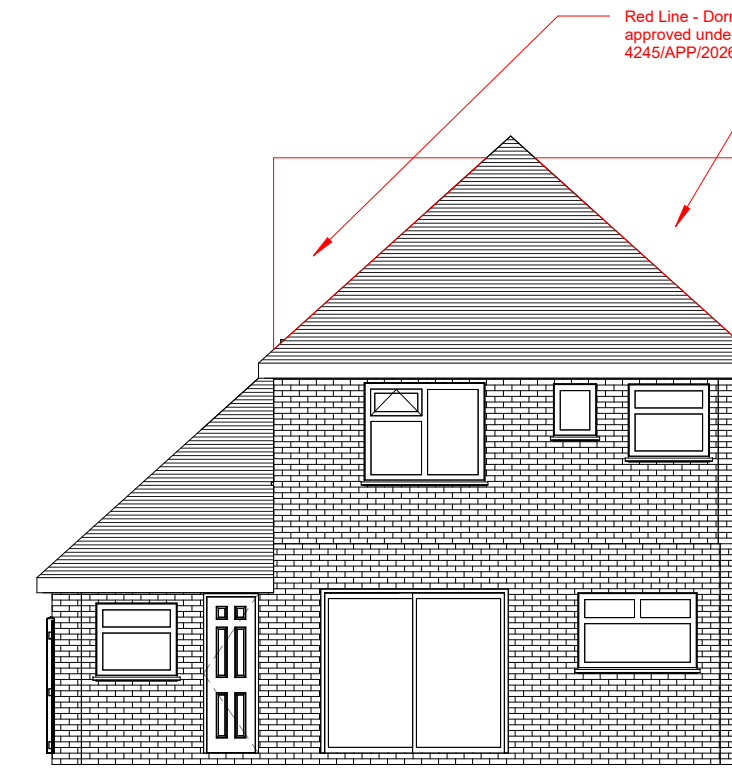
7 Rear Elevatin 1 : 100
