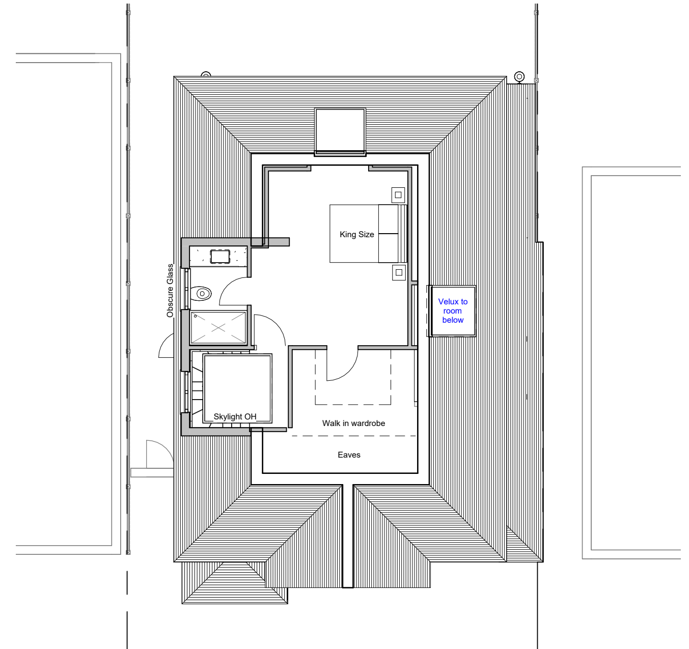
4 Second Floor 1 : 100
