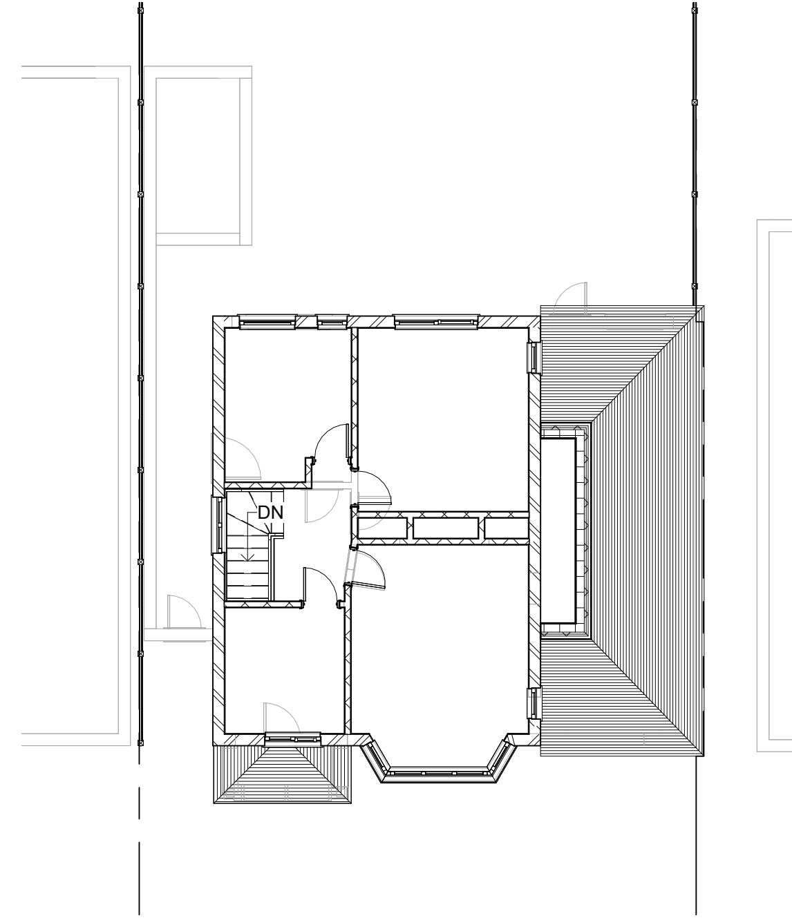
3 First Floor 1 : 100
