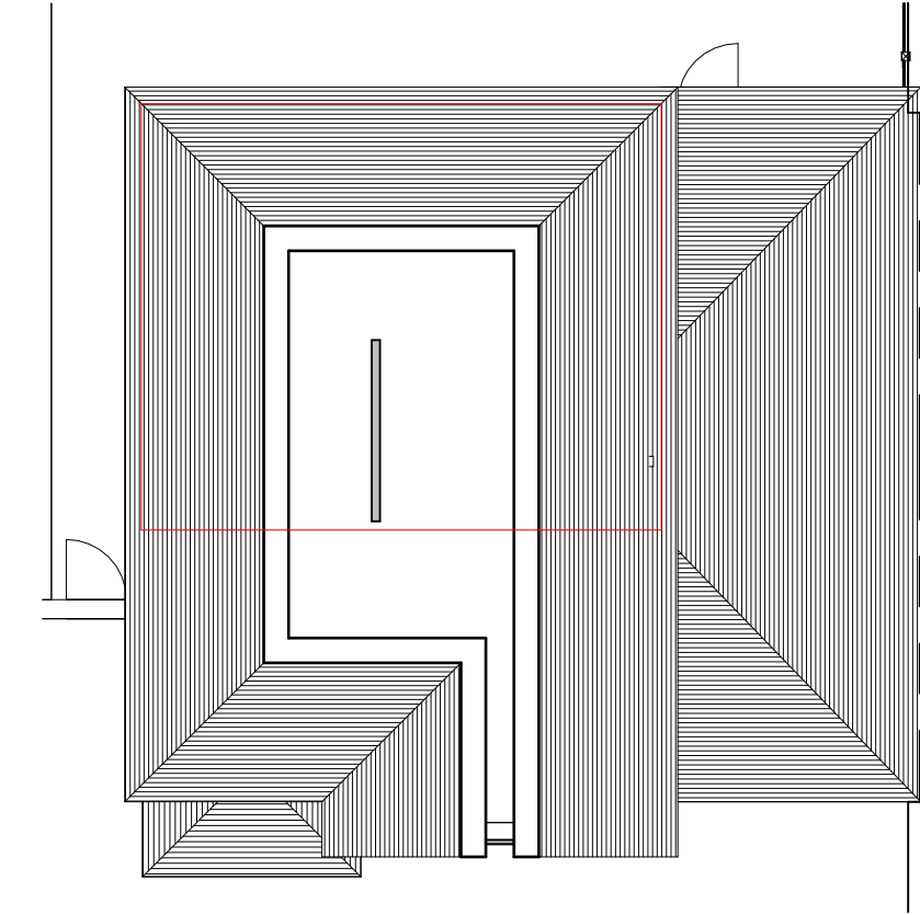
4 Second Floor 1 : 100
