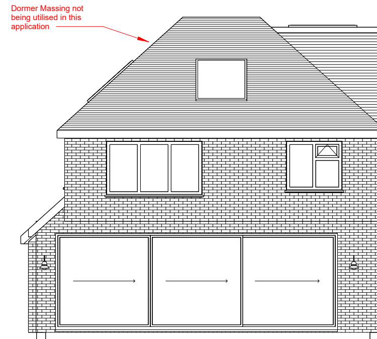
7 Rear Elevation 1 : 100
