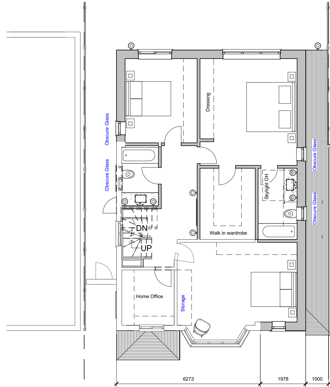
3 First Floor 1 : 100
