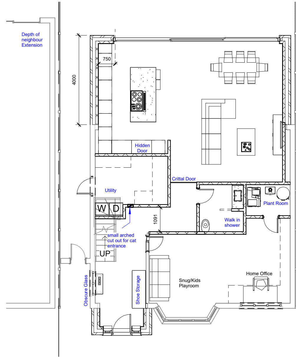
2 Ground Floor 1 : 100
