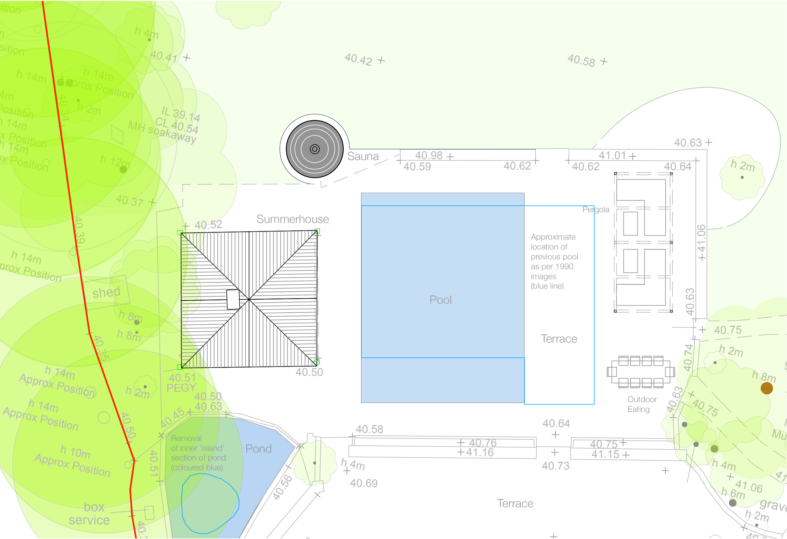
Proposed Pool Area Roof Plan Scale 1:100
