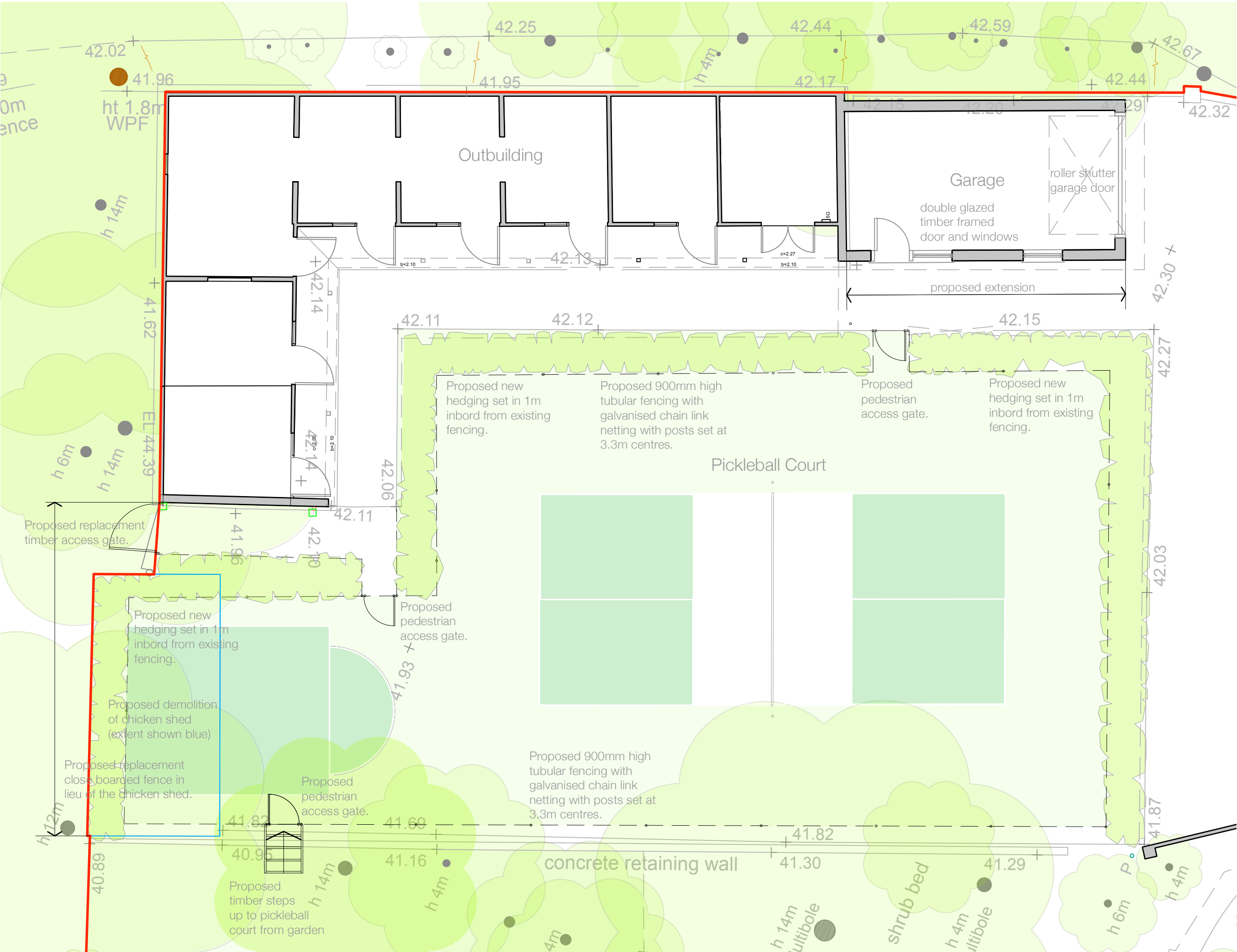
Proposed Plan Garage + Pickleball Court Scale 1:100
