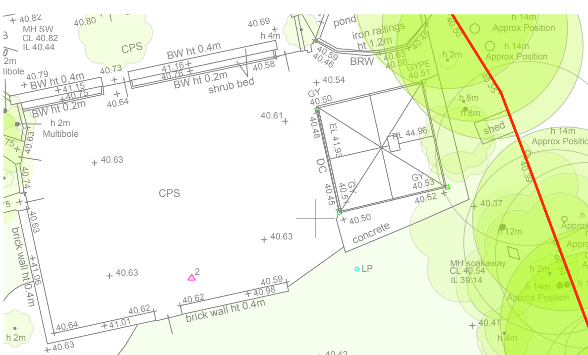
Existing Roof Plan - Pool Building
