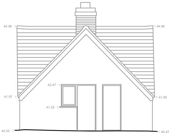
Existing Rear Elevation Scale 1:100
