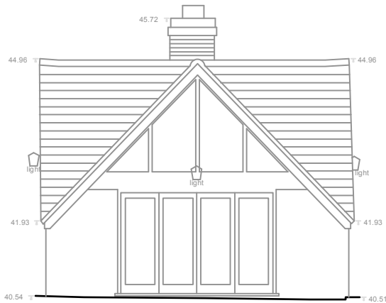
Existing Front Elevation Scale 1:100
