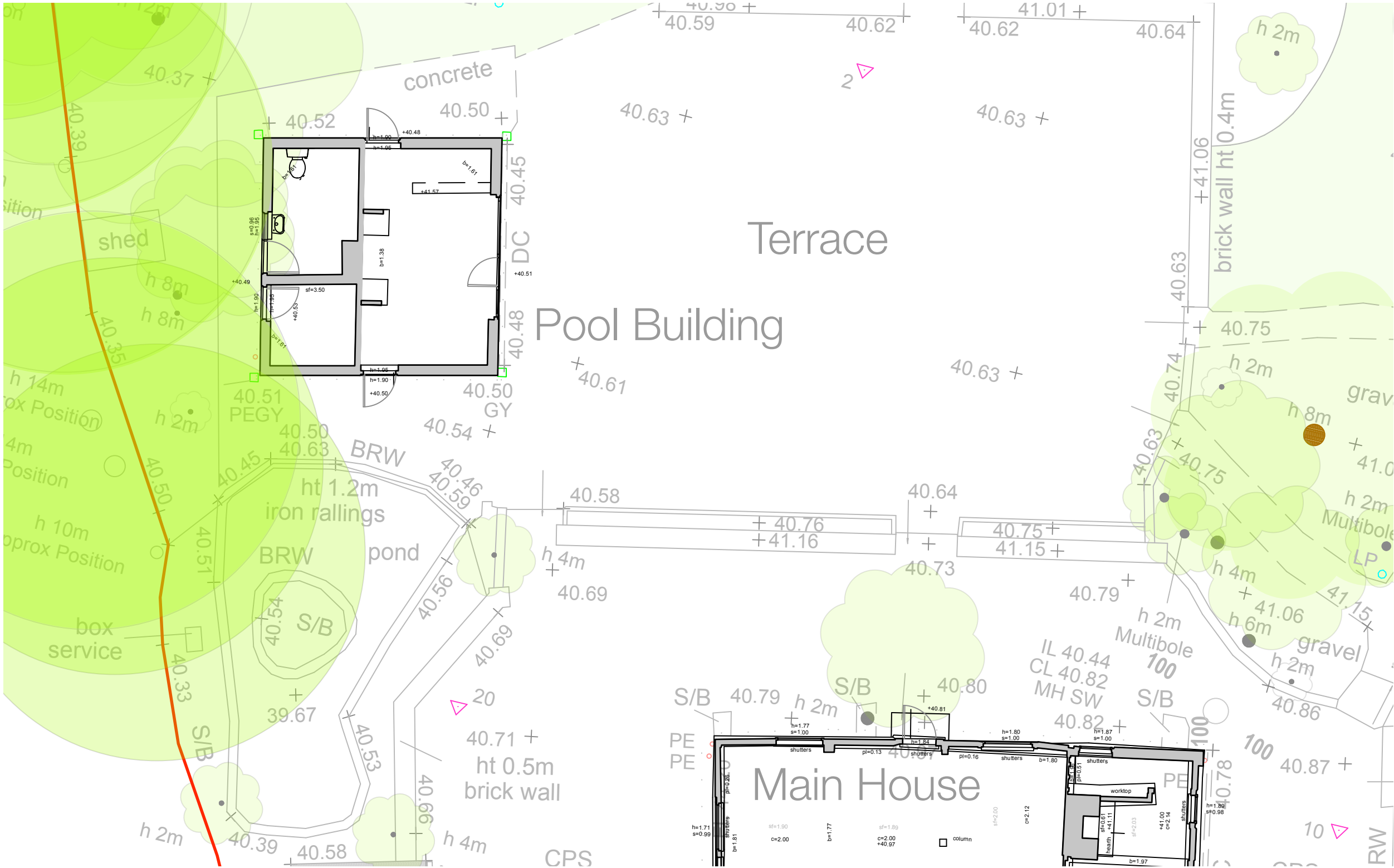
Existing Ground Plan - Pool Building Scale 1:100
