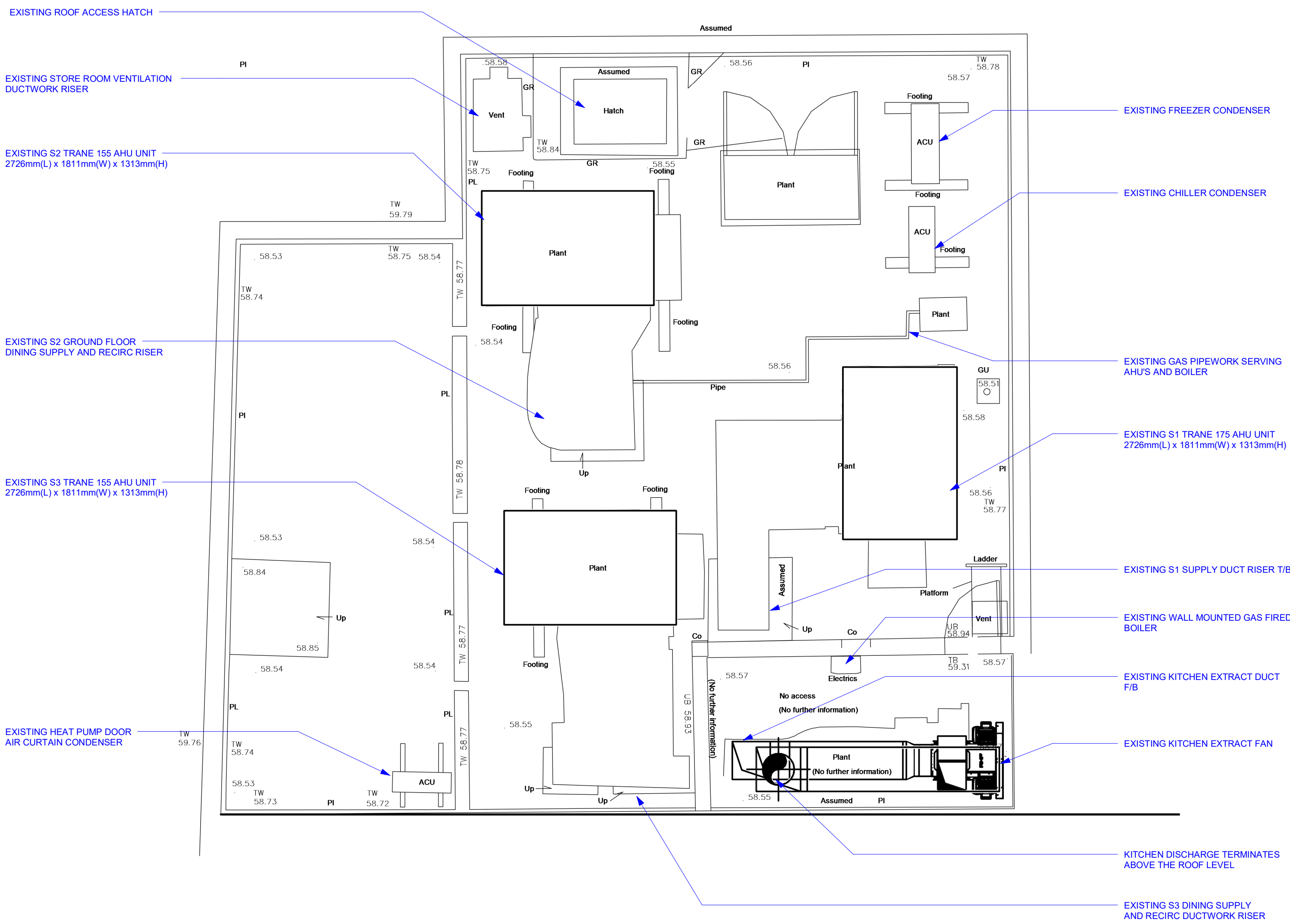
2 Existing Roof 1 : 50
