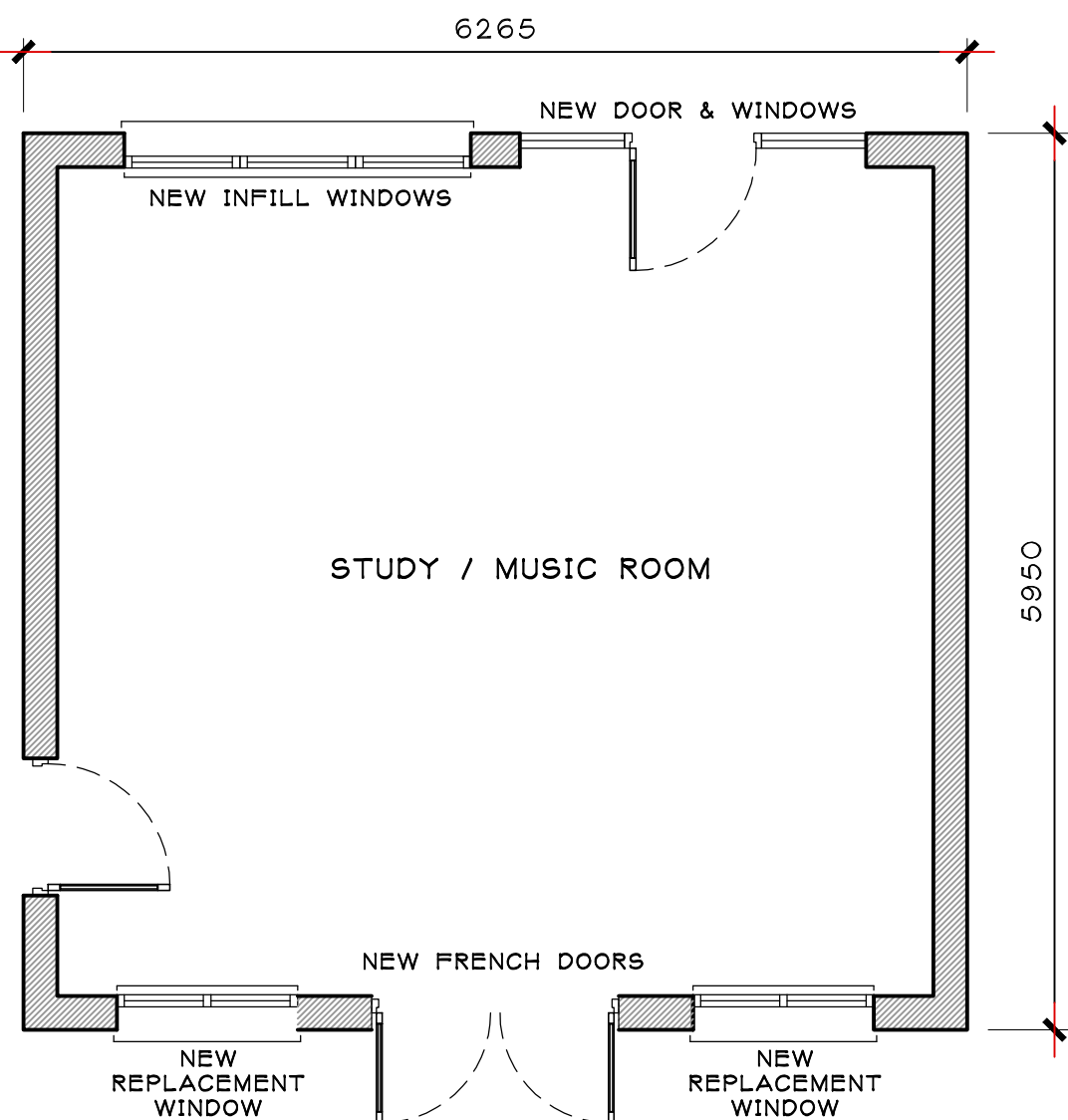
1 FLOOR PLAN SCALE = 1:50
