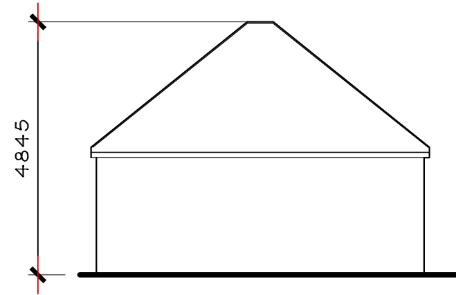
5 RIGHT ELEVATION SCALE = 1:100
