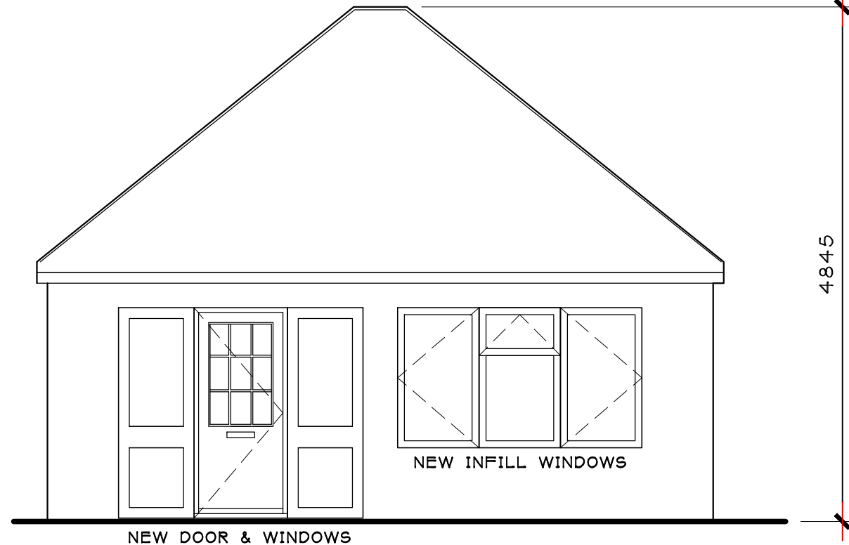
2 FRONT ELEVATION SCALE = 1:50
