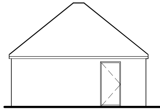
4 LEFT ELEVATION SCALE = 1:100
