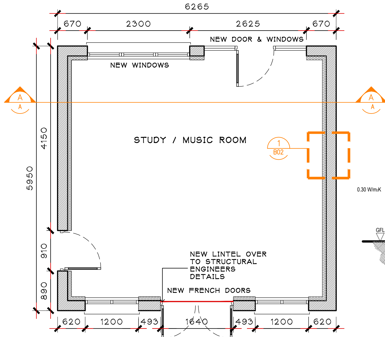
1 FLOOR PLAN SCALE = 1:50
