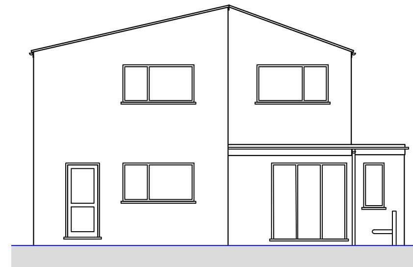
○ Rear Elevation 1 : 1 0 0
