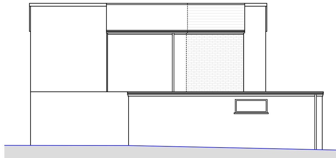
○ Side Elevation 1 1 : 1 0 0
