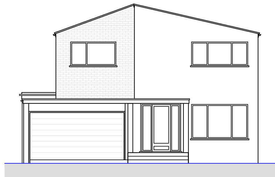
○ Front Elevation 1 : 1 0 0
