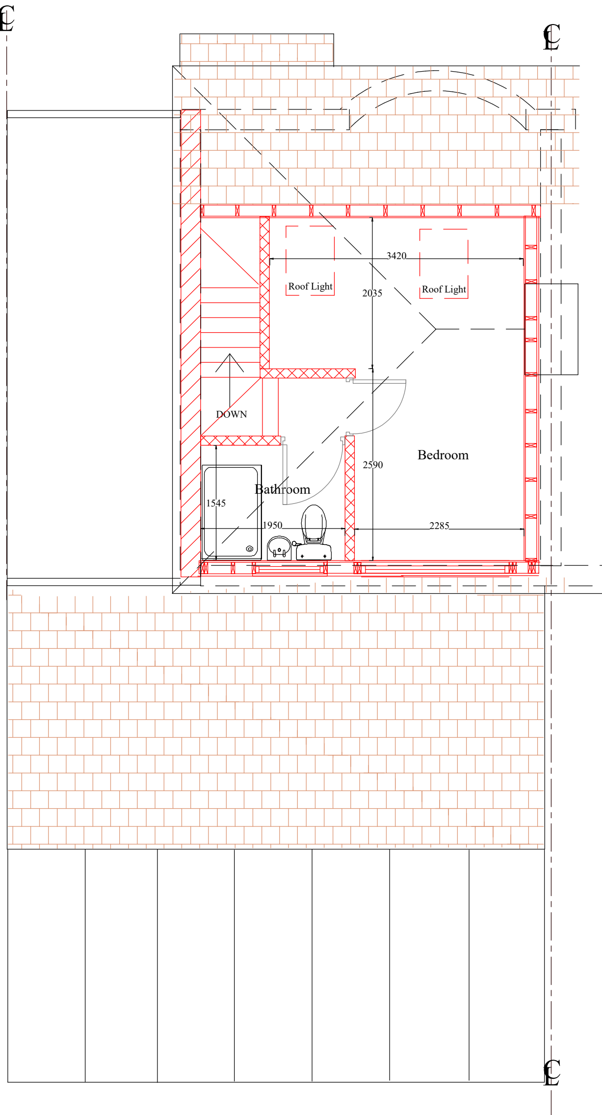
PROPOSED LOFT FLOOR PLAN
