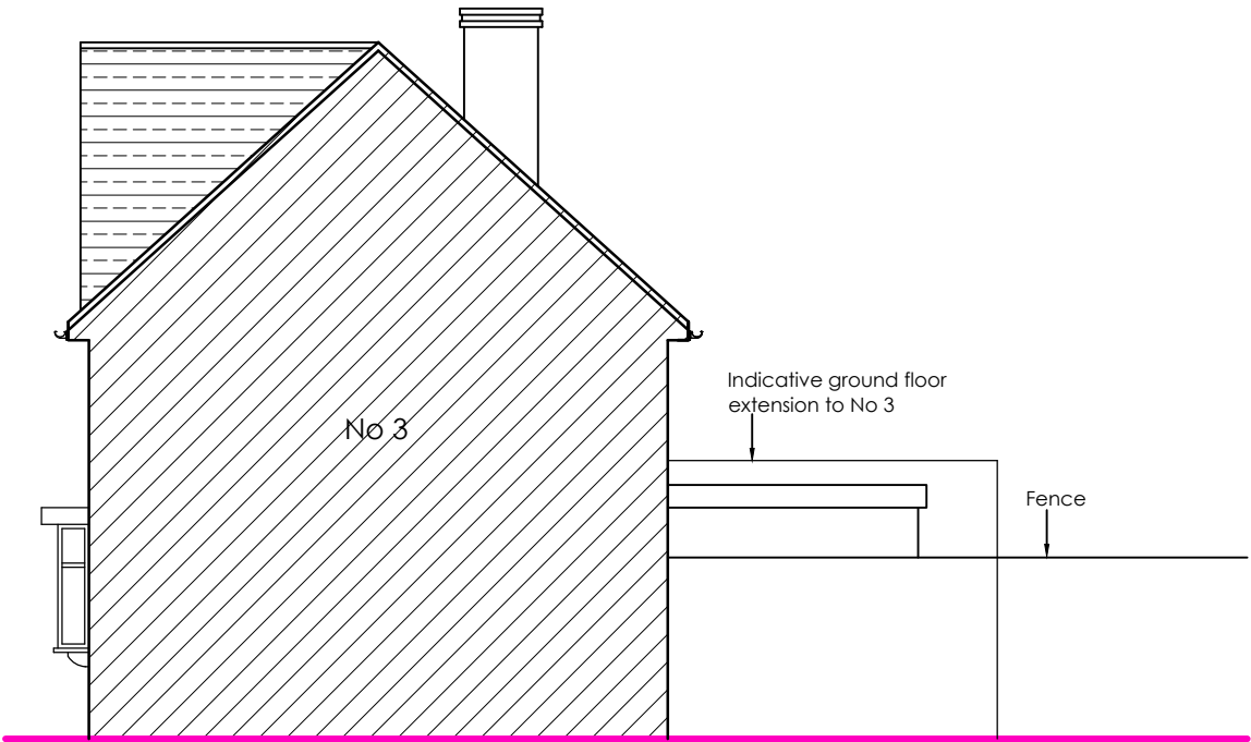
SIDE ELEVATION No 3
