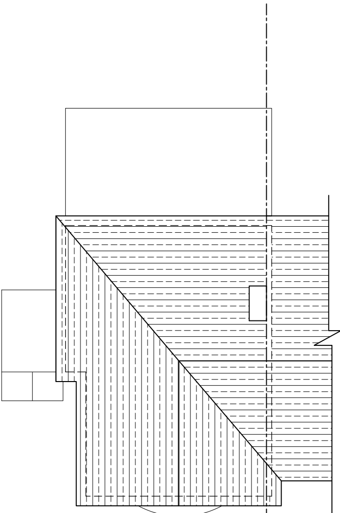
ROOF PLAN
