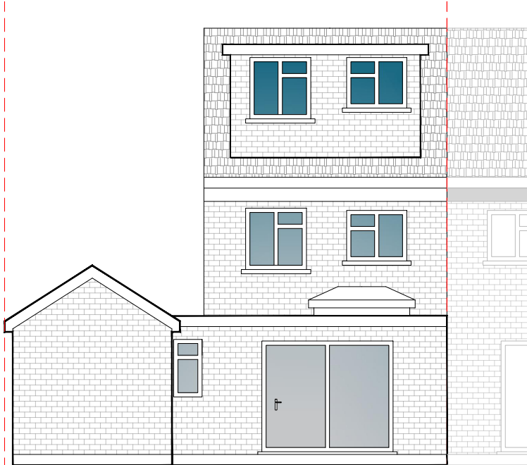
Proposed Rear Elevation Plan
