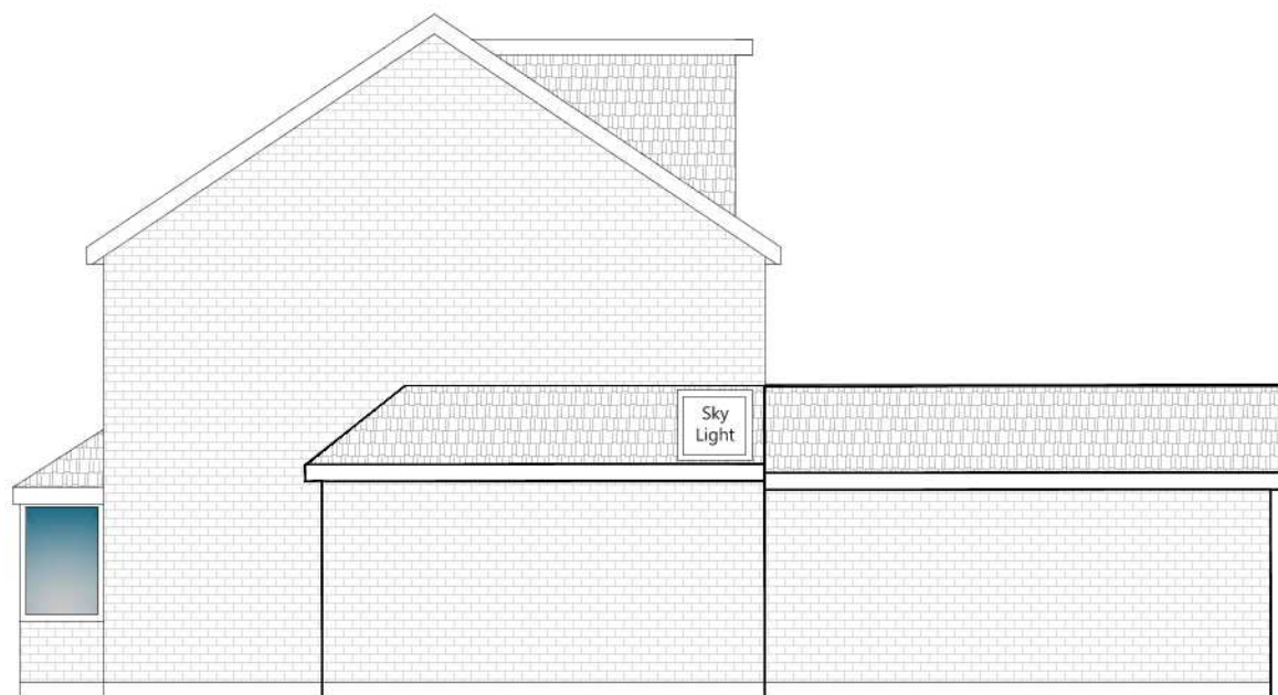
Proposed West Facing Side Elevation
