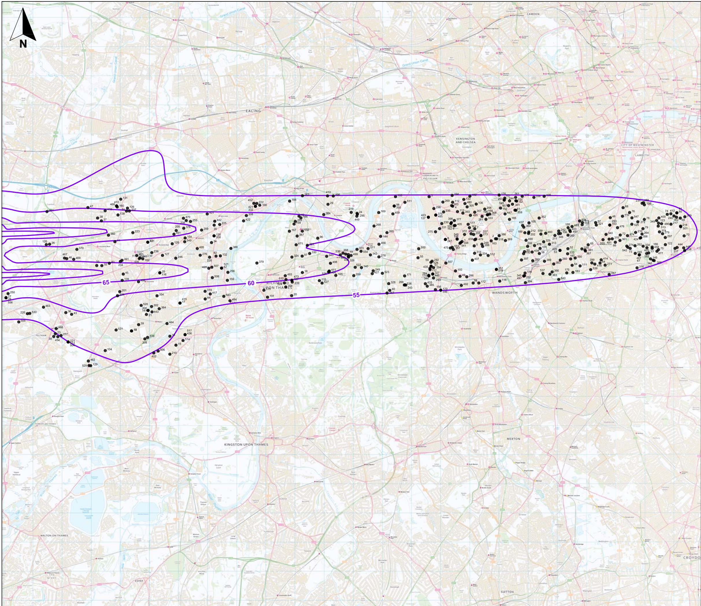
Figure G.30 E - East Air Noise, 2015 Without Cranford, Lden, Westerly Mode (78%W/22%E) with Education
