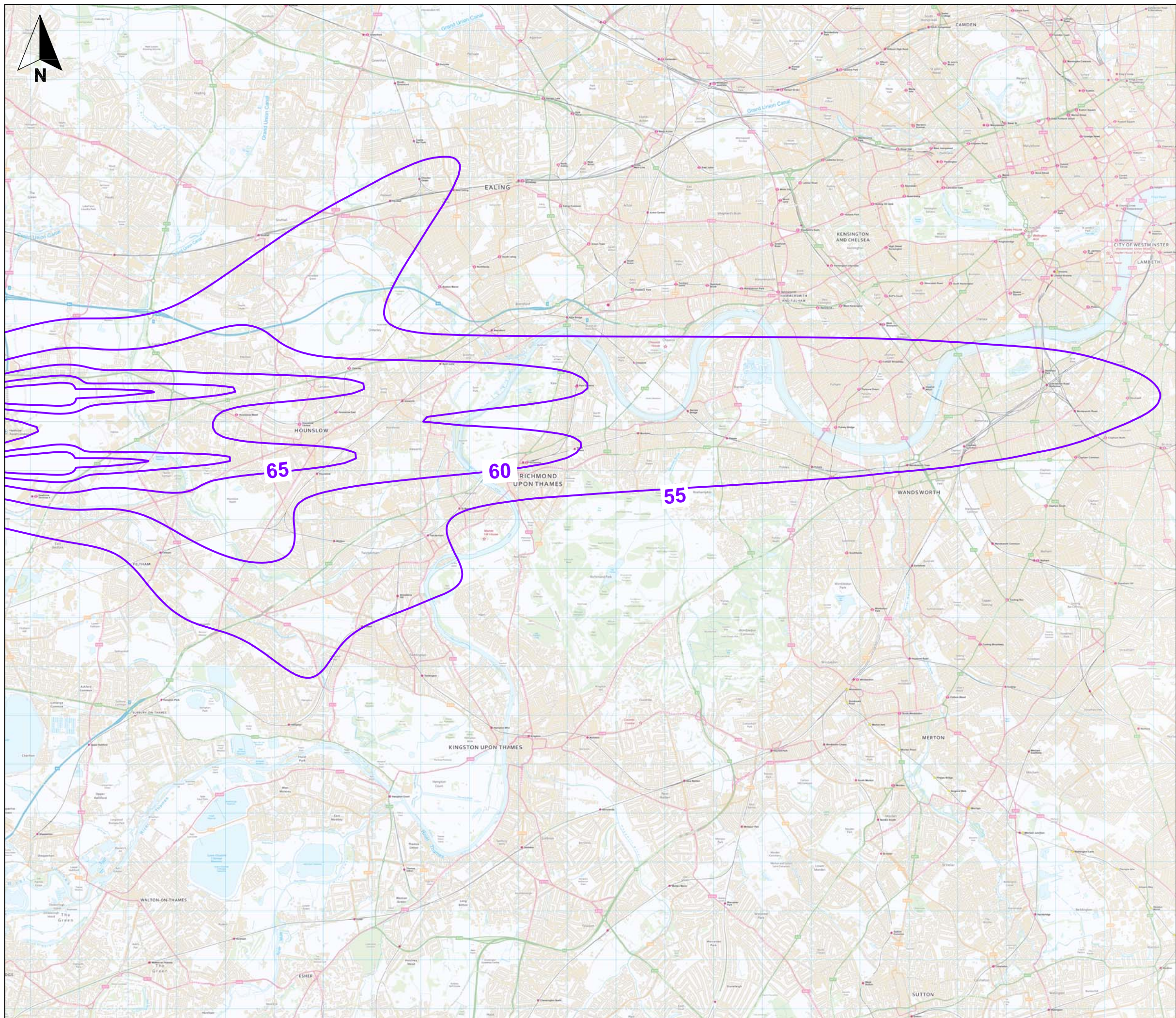
Figure G.28 - East Air Noise, 2015 Without Cranford, Lden, Easterly Mode (60%W/40%E)
