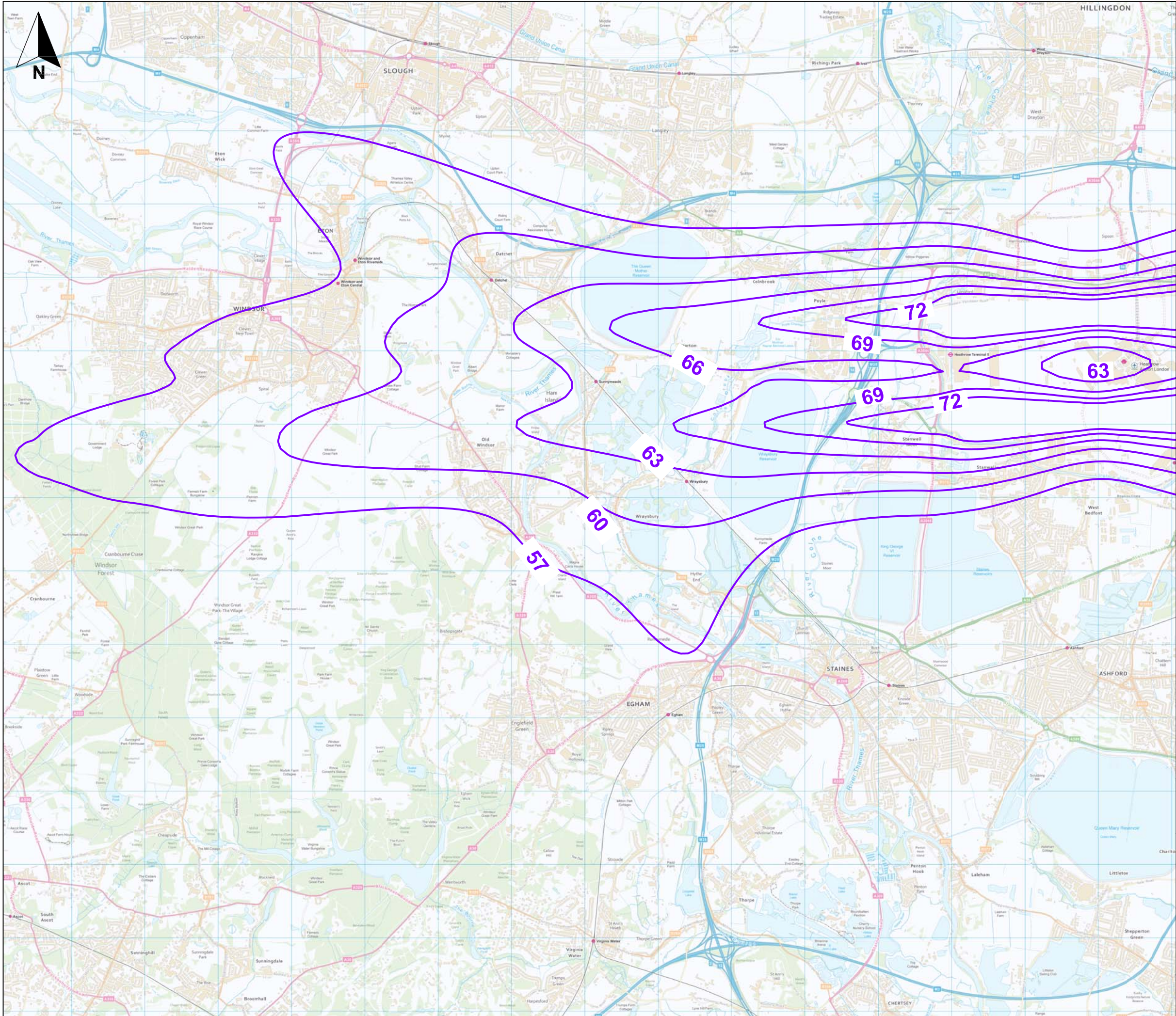
Figure G.20 - West Air Noise, 2015 Without Cranford, LAeq,16hr Easterly Mode (60%/W/40%E)
