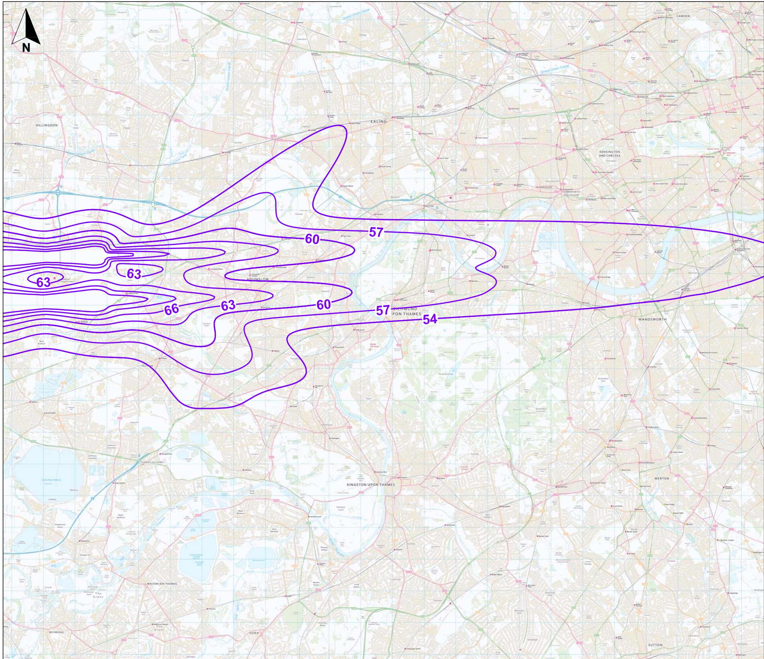
Figure 6.2 - East Air Noise, 2011 Standard Mode Contours, LAeq,16hr - With Cranford
