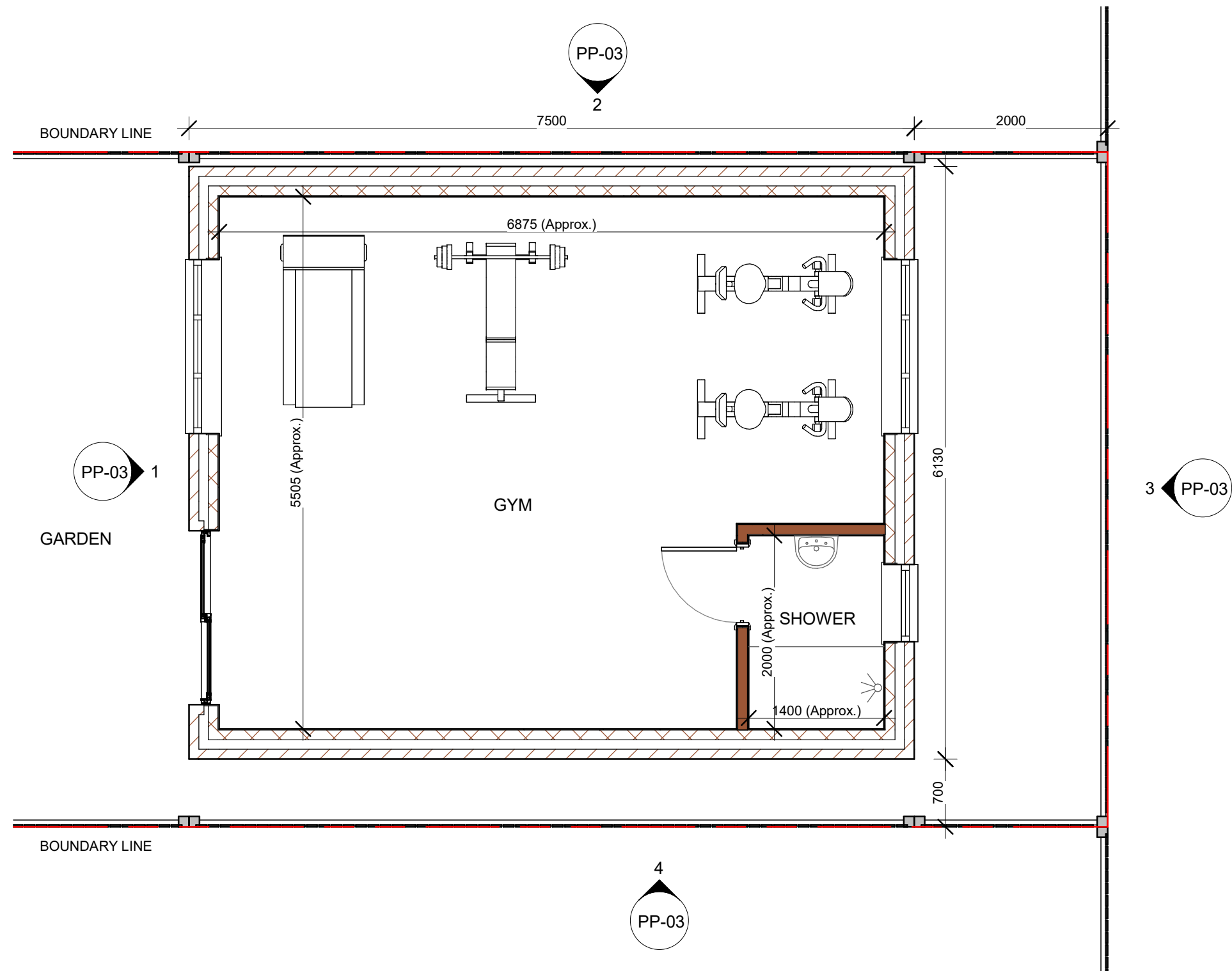
PP-PROPOSED GROUND FLOOR PLAN
