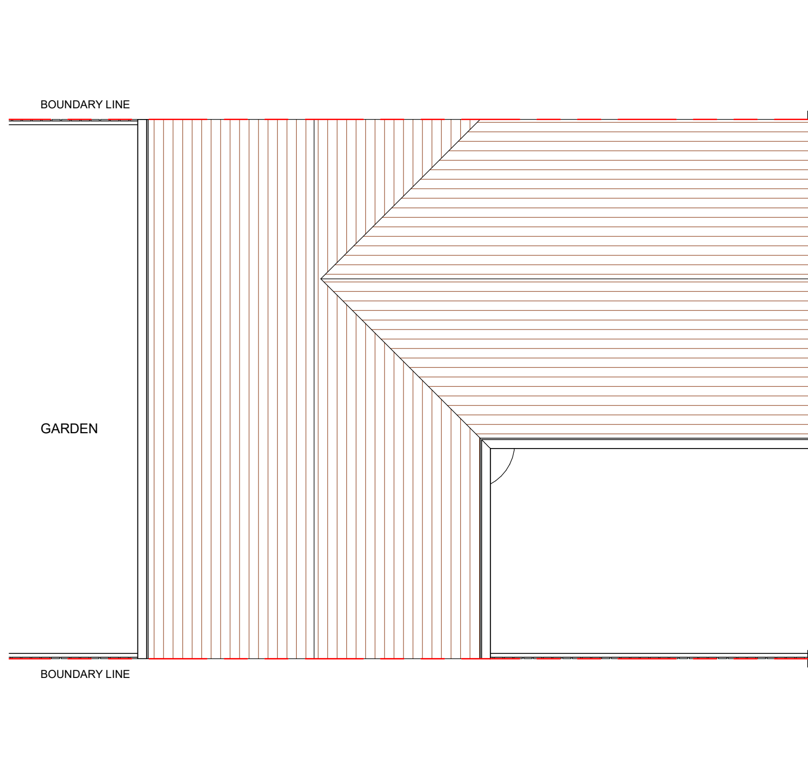
PP-PROPOSED ROOF TOP PLAN 1 : 50
