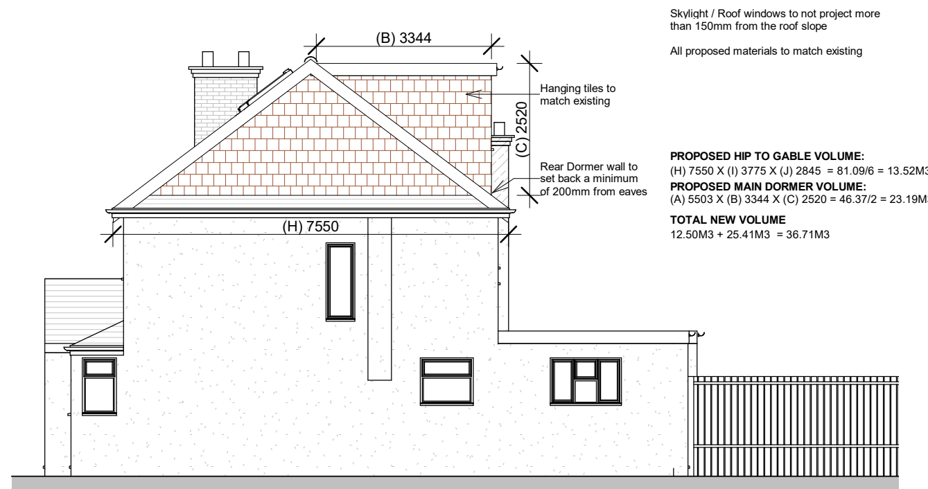
PP-PROPOSED SOUTH SIDE ELEVATION 1 : 100
