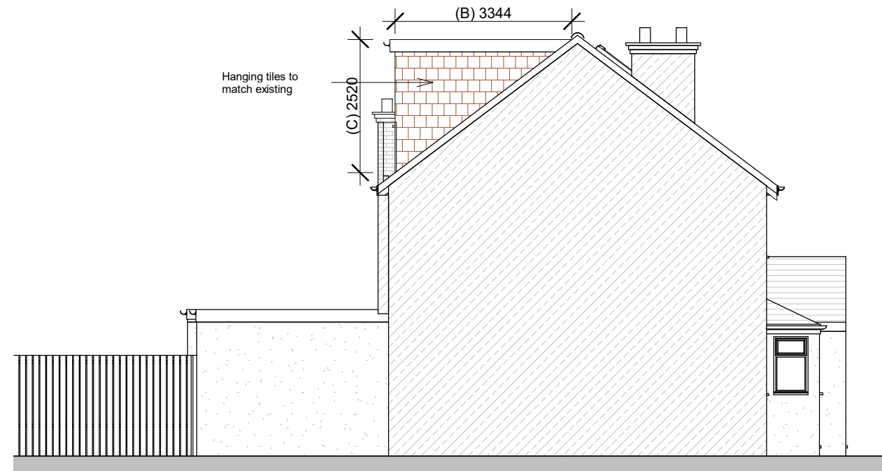
PP-PROPOSED NORTH SIDE ELEVATION 1 : 100
