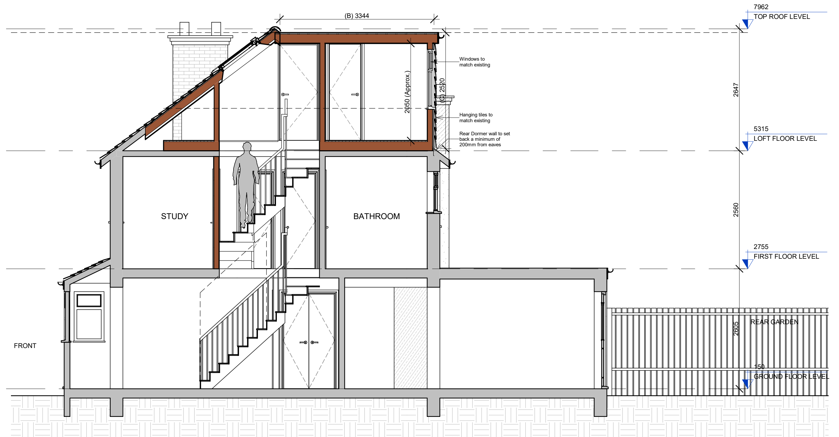
PP-PROPOSED SECTION A 1 : 50
