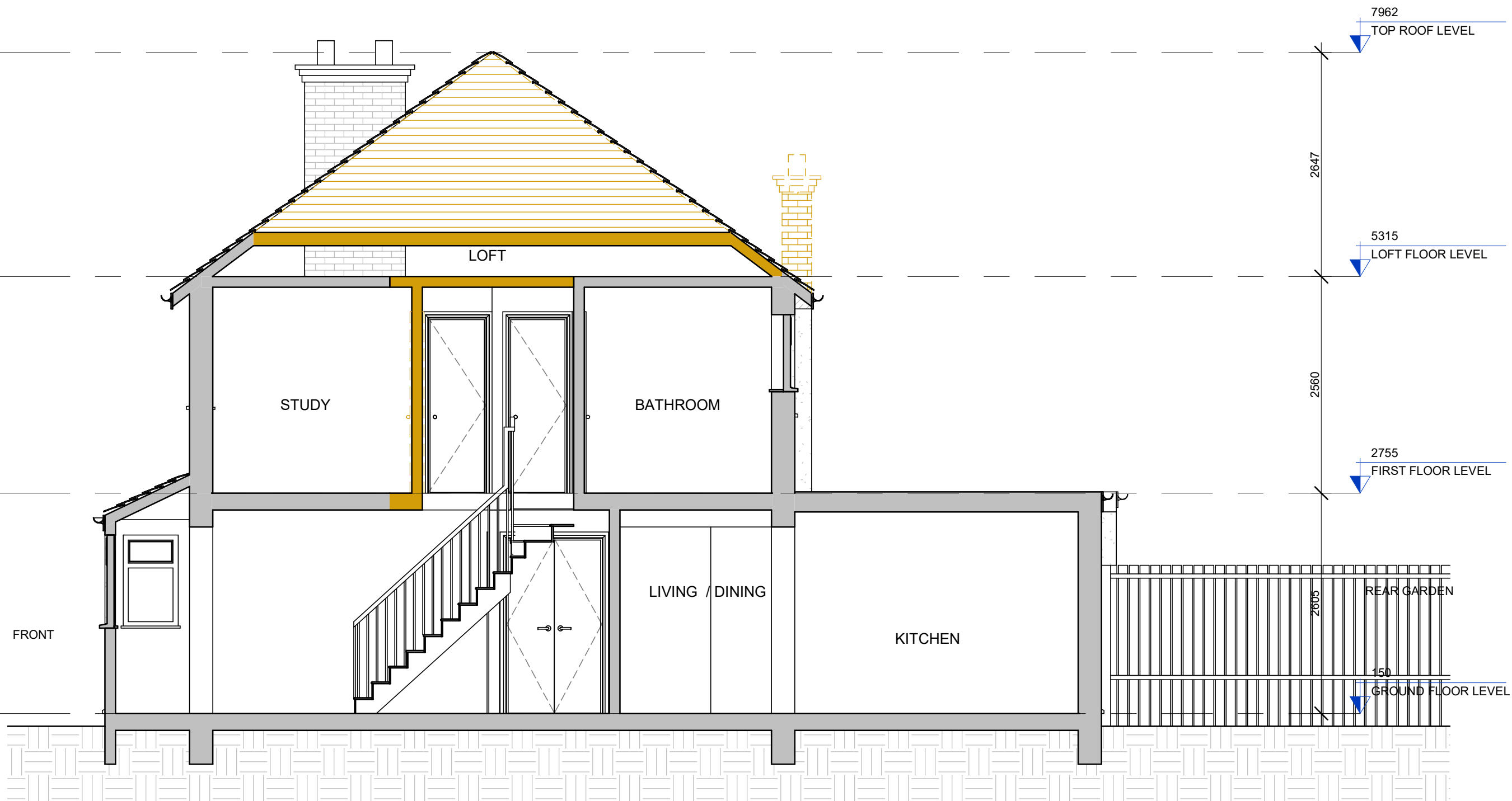
PP-EXISTING SECTION A 1 : 50
