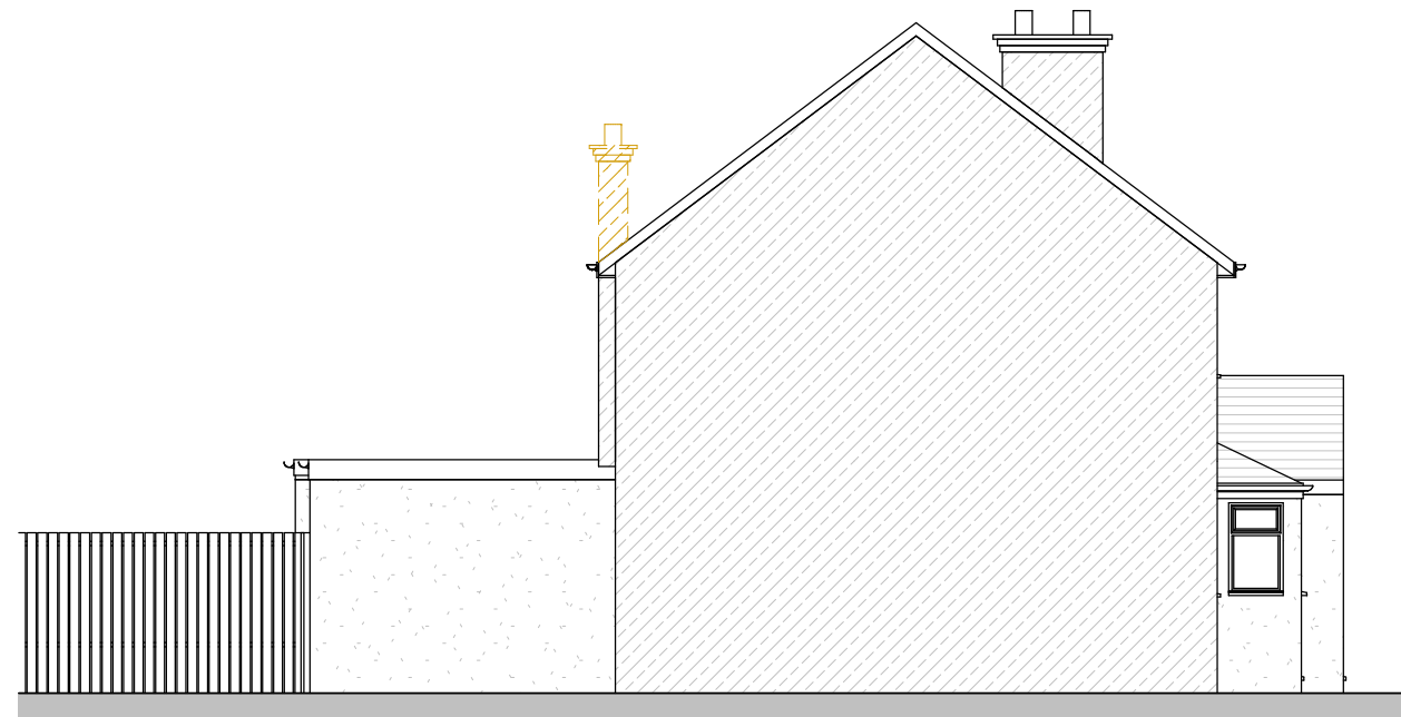
PP-EXISTING NORTH SIDE ELEVATION 1 : 100
