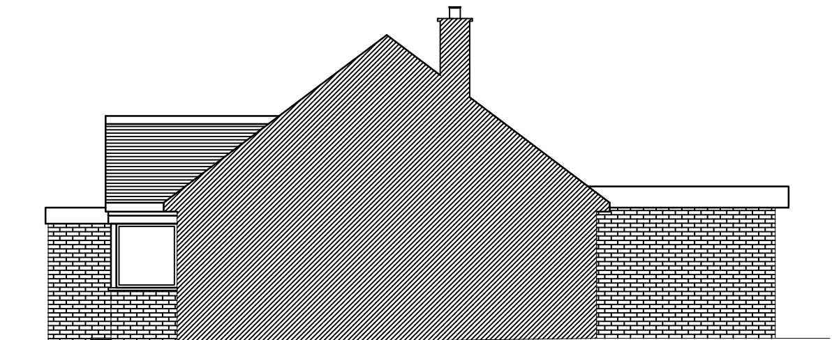
SIDE ELEVATION EXISTING (AS VIEWED FROM NO:4)
