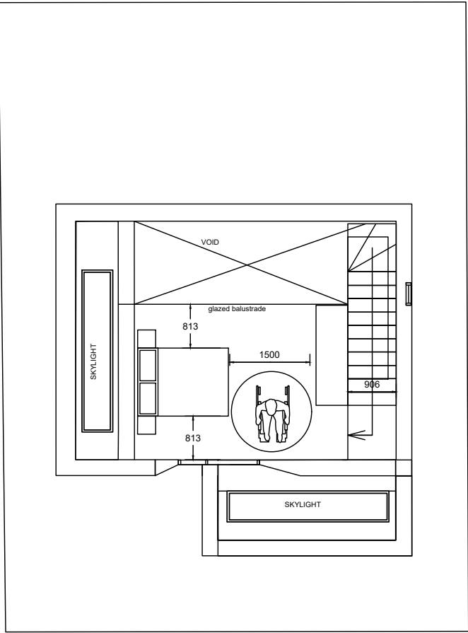
Mezzanine plan
