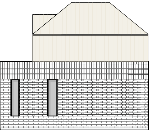
Proposed Left Side Elevation
