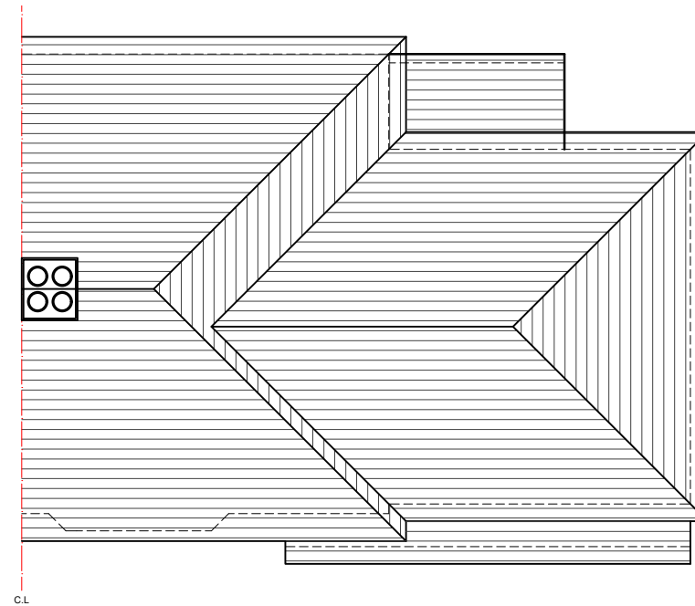
03 - ROOF PLAN
