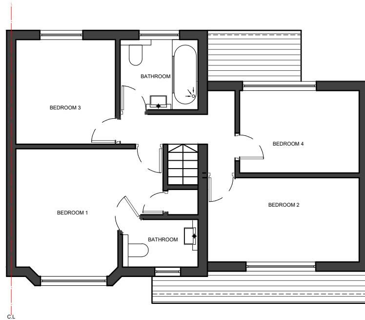
02 - FIRST FLOOR PLAN
