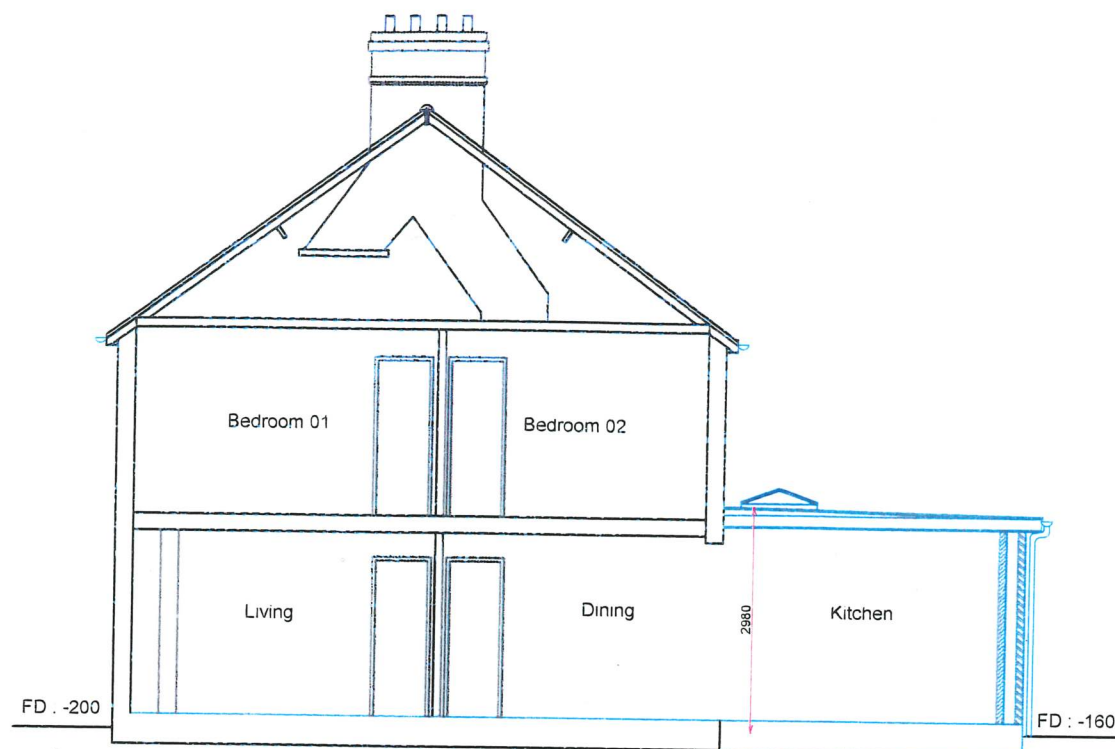
PROPOSED SECTION
