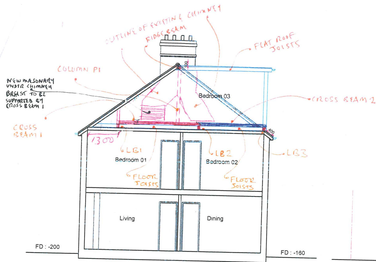
PROPOSED SECTION
