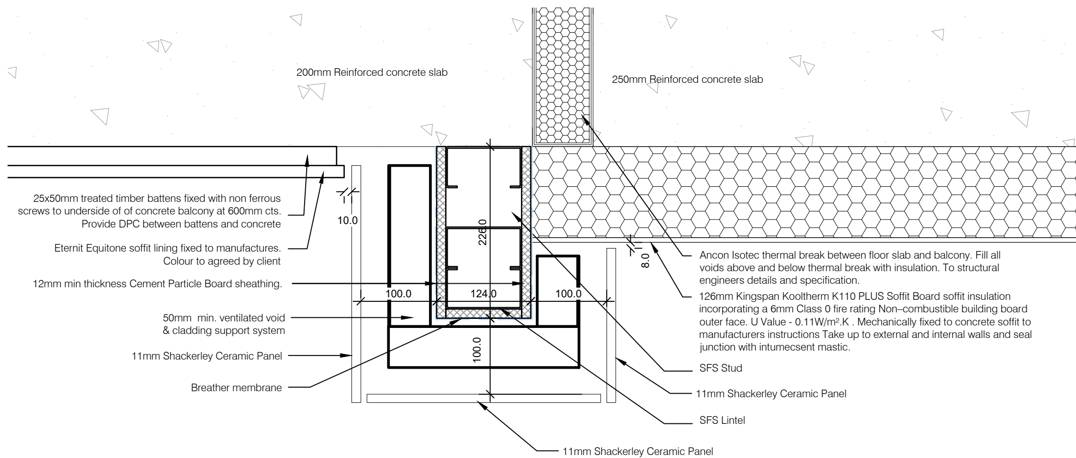
1 Undercroft Detail Scale 1:5
